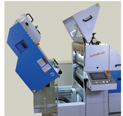
Easy access for the change of the punching plates
